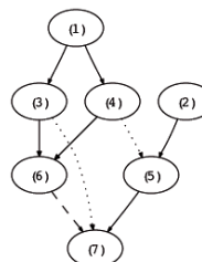
PDG of Program 1
