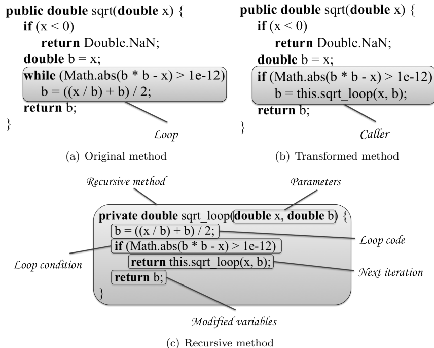
Figure 2: while -loop transformation
