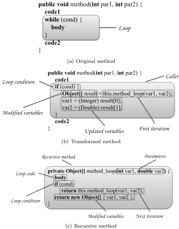
Figure 1: while -loop transformation
