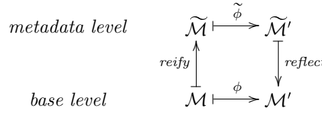
Figure 2.3: Reflection.
