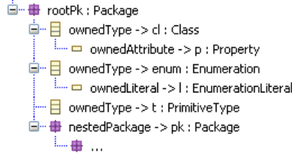
Figure 6.5: Tree structure of a metamodel \widetilde{\mathcal{M}} : \text{MOF} .
