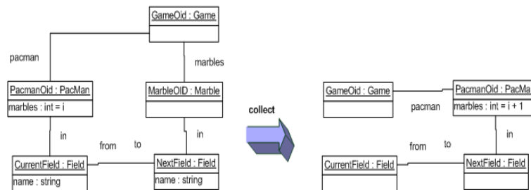
Figure 9.20: Graphical representation of the collect production rule of the PacMan game.
