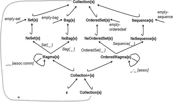
Figure 6.2: Subsort Structure of our Specification of the OCL Type System.
